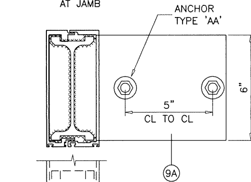
CONCRETE OR METAL STRUCTURE DETAIL '1' AT JAMB
