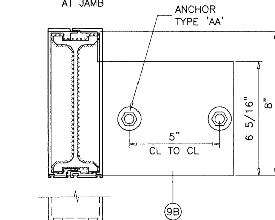
CONCRETE DETAIL '1' AT JAMB
