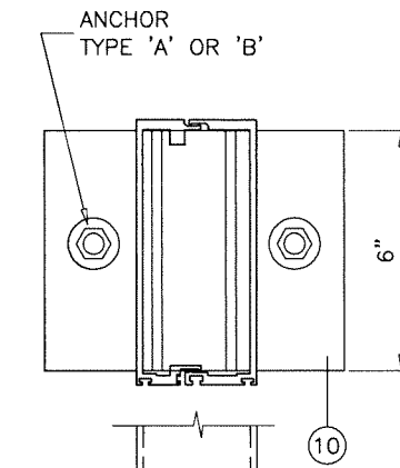
CONCRETE OR METAL STRUCTURE DETAIL '2' AT MULLION
