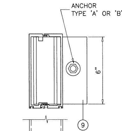
CONCRETE OR METAL STRUCTURE DETAIL '1' AT JAMB
