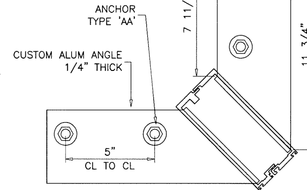
DETAIL '3' AT 90° CORNER MULLION
