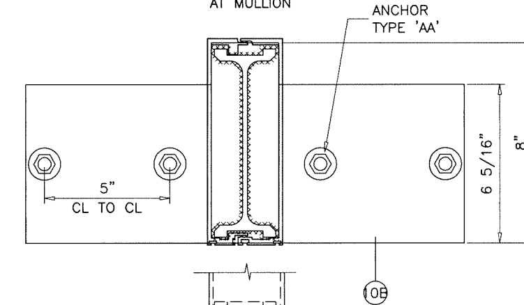
CONCRETE DETAIL '2' AT MULLION
