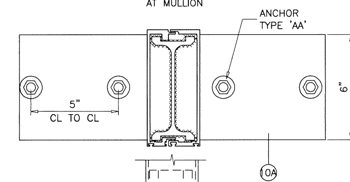
CONCRETE OR METAL STRUCTURE DETAIL '2' AT MULLION
