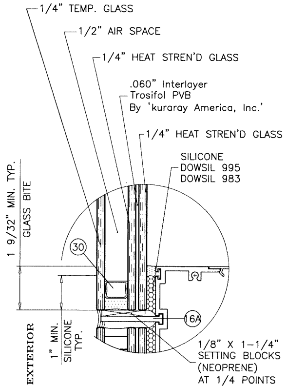
GLASS TYPE 'E1'
